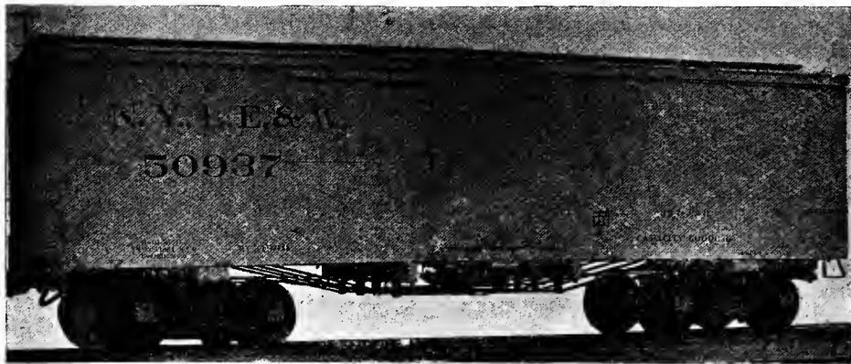
Fig. 3. BOX CAR. NEW YORK, LAKE ERIE & WESTERN RAILROAD. Length, 34 ft. Capacity, 60,000 lbs. Weight, 31,000 lbs. Equipped with Air Brakes and Rigid Diamond Trucks.
